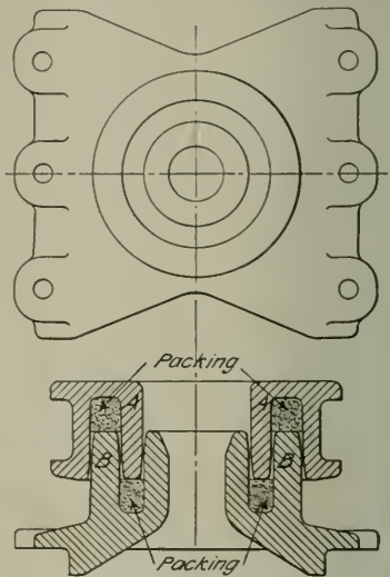
ARTICULATED COUPLING BETWEEN TRUCKS.
